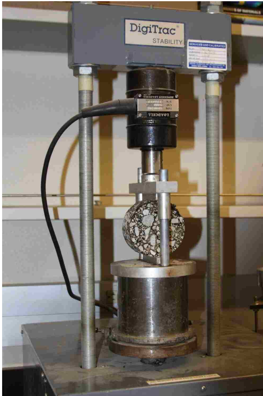
Figure 4.2. IDT Testing Apparatus
